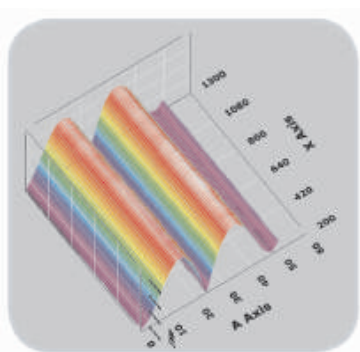
Measurement Tool Output: 3D Graph of Actual B Field
